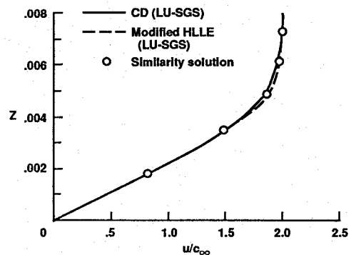
Fig. 1 Comparison of computed laminar boundary-layer profiles on a flat plate between the central difference and the upwind algorithms, M_\infty = 2.0 and Re = 10^6 .
