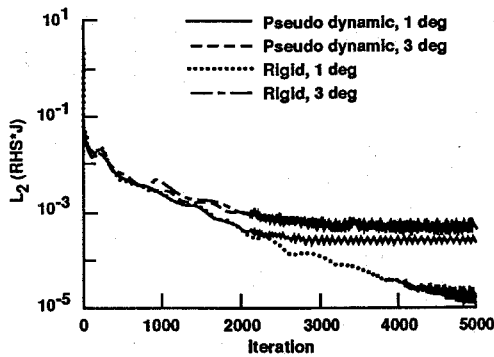
Fig. 13 Comparison of convergence history for flexible and rigid wing cases, M_\infty = 0.85 , Re_c = 0.6 \times 10^6 , and \alpha = 1 and 3 deg.
